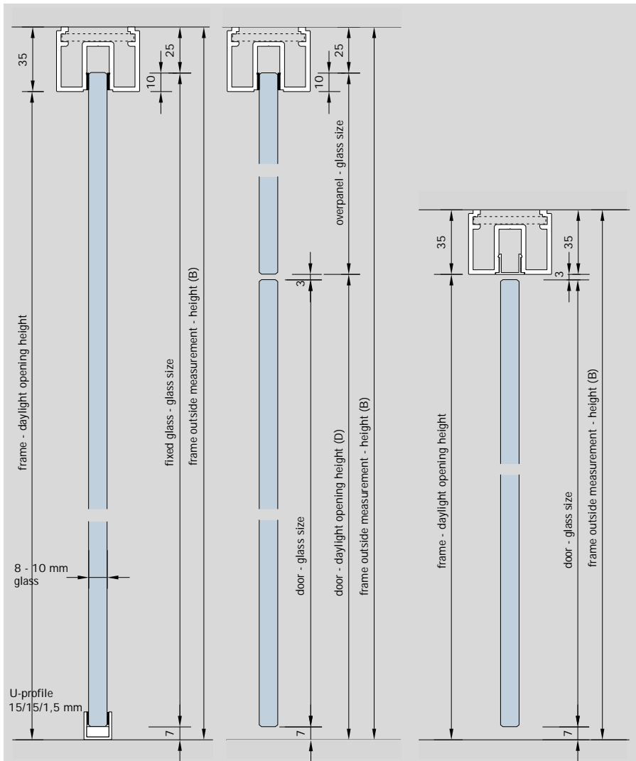
sectional cut / fixed glazing
