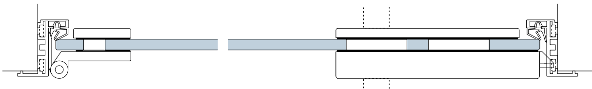
Deubl AT 23 E with DORMA special hinge Art. no. 11.294 resp. 12.050, lock Studio Rondo / Classic
