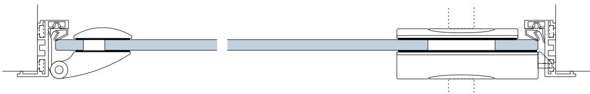
Deubl AT 23 E with DORMA special hinge ARCOS Art. no. 25.450, lock ARCOS Office
