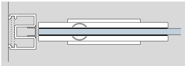
plan DORMA Universal patch fitting
