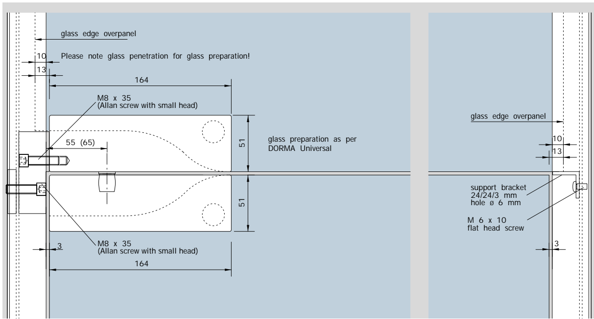
view DORMA Universal patch fitting
